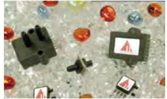
An assortment of sensors features the 0.025-in. H20 Full Scale A-package (top) and a range of mini packages. The A-package accurately reads exceedingly low pressures. The devices are for drug delivery, respiratory, and similar applications where physical size is not a constraint. Mini packages target devices requiring a smaller sensor such as for measuring oxygen in a medical device.
