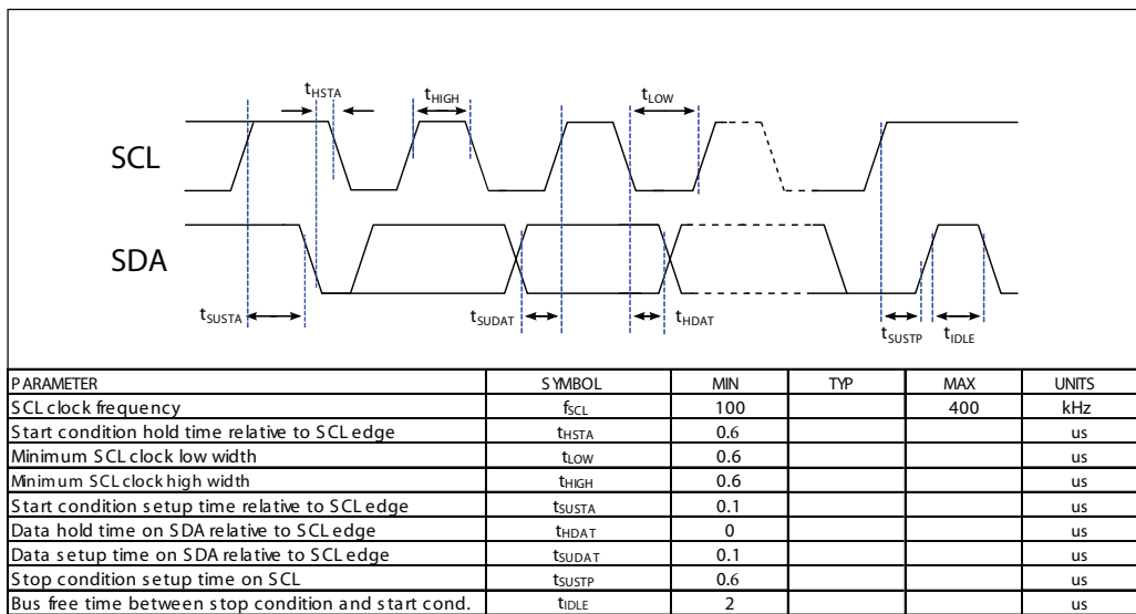
Figure 7 - I2C Timing Diagram
