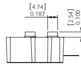
C- Two Ports Cut 0.100" Configuration
