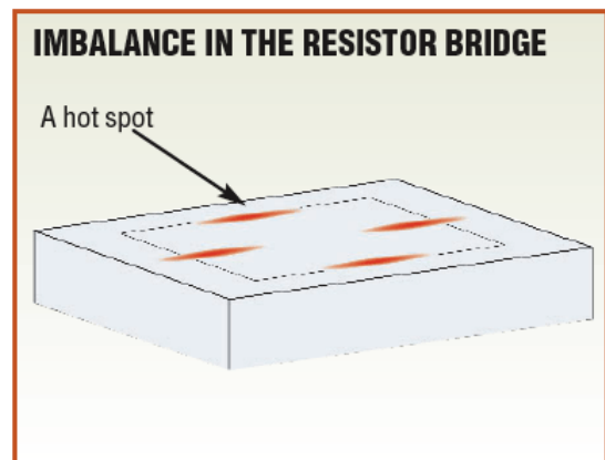
Thermal hot spots on the die and diaphragm surface (orange lines) cause an imbalance in the resistor bridge.
