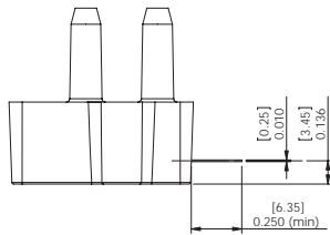
F- Flat (Straight) Configuration
