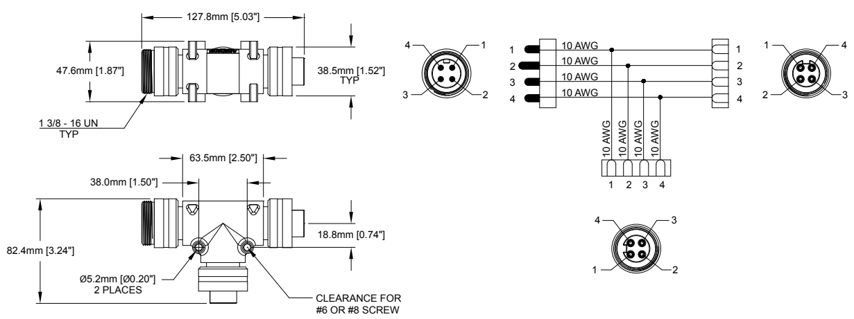
FIG 14: Tee, 4 Position
