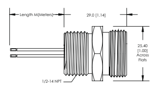
FIG 12: Female, Mini, Receptacle, Thick, Internal Threads
