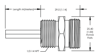
FIG 11: Male, Micro, Receptacle, Thin, External Threads
