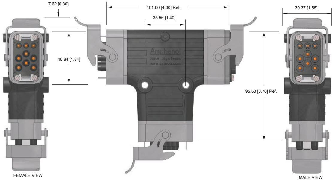
FIG 7: Hybrid Tee, 600V, 9 Position
