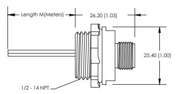
FIG 13: Female, Mini, Receptacle, Thin, Internal Threads
