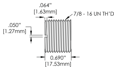
FIG 13: Threaded Union
