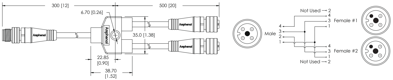
FIG 7: Male to Female, Splitter, Straight - (1) 4 Pos. to (2) 4 Pos.
