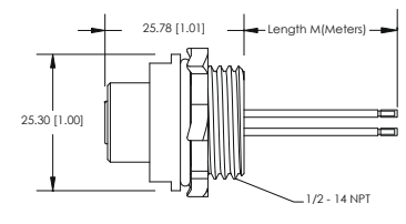
FIG 16: Female, Terminating Plug, Straight, 5 Position
