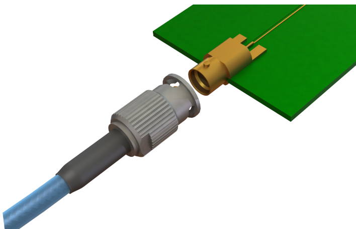
Figure 1: Female QB Cable Assembly to Male Edge Launch PCB Connector, Unmated
