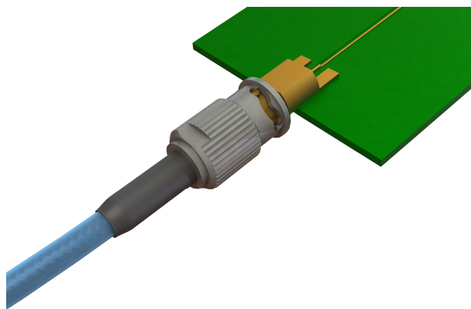
Figure 2: Female QB Cable Assembly to Male Edge Launch PCB Connector, Mated
