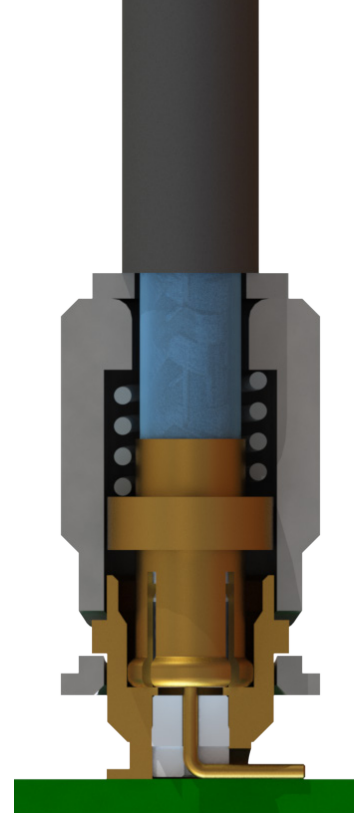
Figure 3: Cut-away view of a mated Female QB Cable Assembly to Male QB PCB Connector
