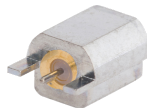
SMPM Male PCB Edge Launch Connector (Back) PN: 3211-60307 and 3211-60308
