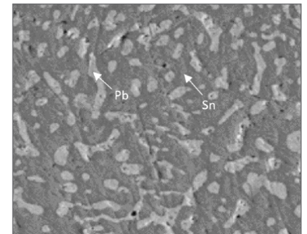
Figure 4: High mag view of solder joint in Figure 3 showing minimal gold in solder
