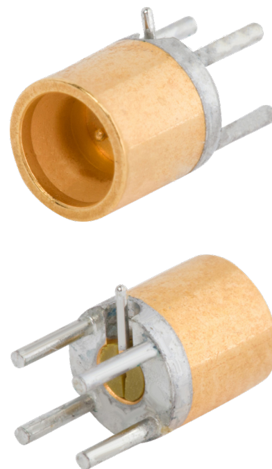
Pre-tinned (De-golded) PCB Connectors PN: 3211-40093 and 3211-40094
