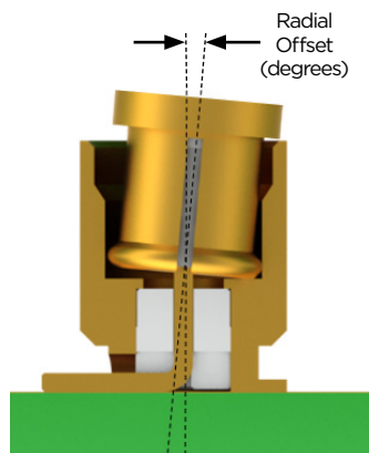
Figure 2: Radial Misalignment Measurement
