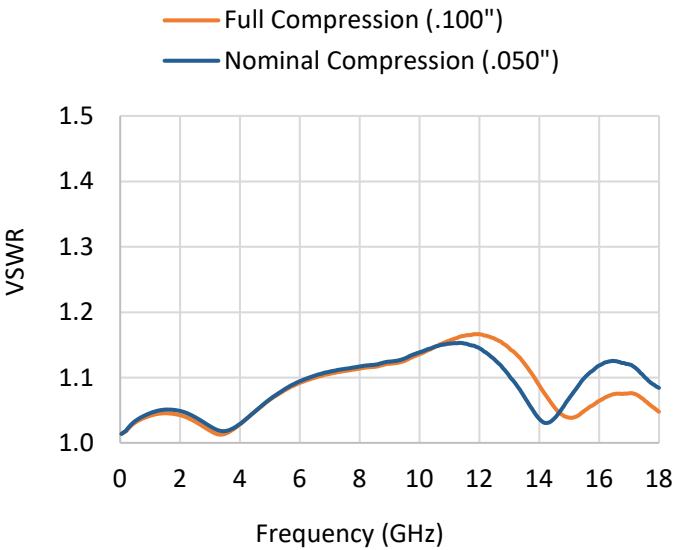
Figure 10: Effect of Compression on Electrical Performance of an SMP Spring Bullet (1112-4146)
