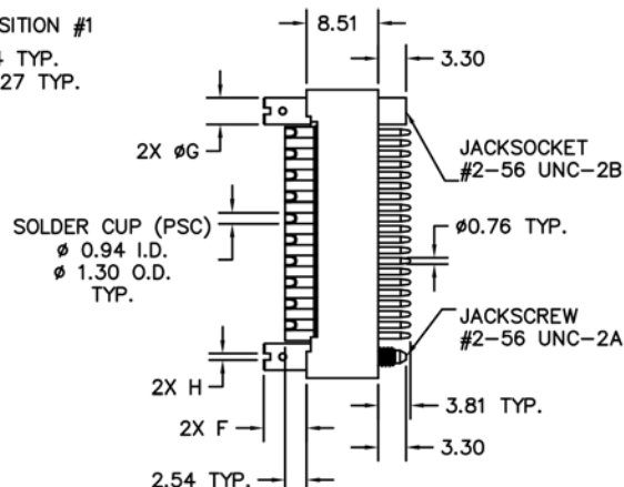
PLUG (WITHOUT EARS) (IW-2P0-20-PSC-JTA)
