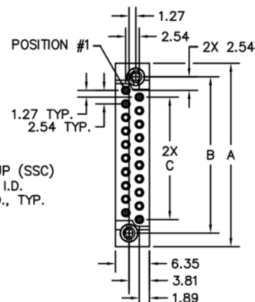
RECEPTACLE (WITHOUT EARS) (IW-2R0-20-SSC-J)
