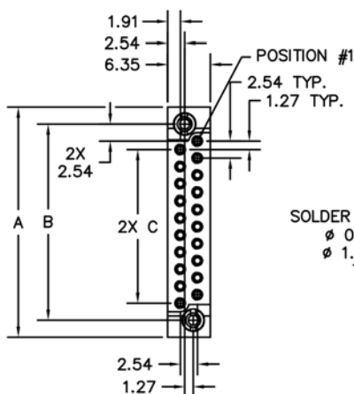
PLUG (WITHOUT EARS) (IW-2P0-20-PSC-JTA)
