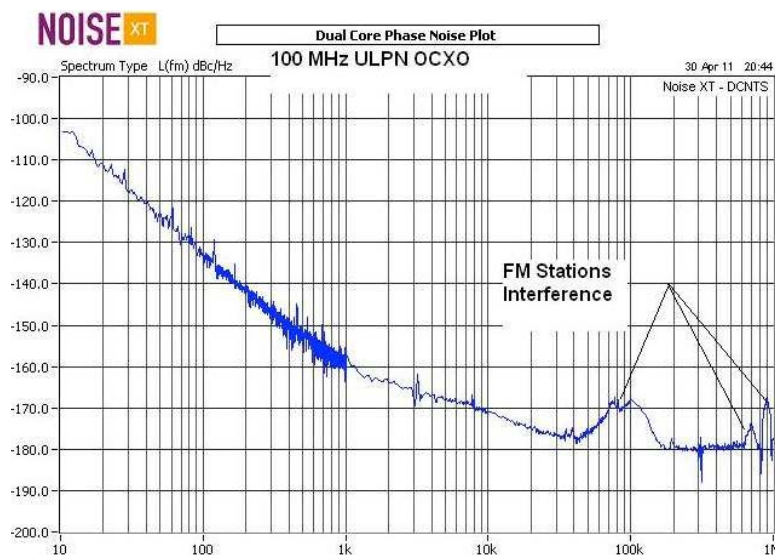
Fig. 3. 100 MHz ULPN OCXO with “bumps” caused by RF pollution.
