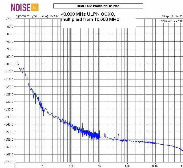
Fig. 12. 40 MHz OCXO, multiplied from 10 MHz
