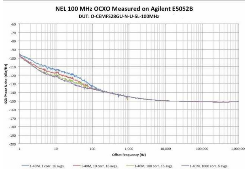
Fig. 13. 100 MHz ULPN OCXO multiplied from 10 MHz, tested on Agilent E5052B with various number of crosscorrelations and averages
