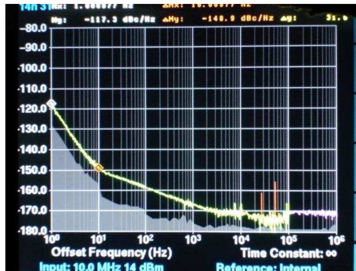
Fig.1. 10 MHz ULPN OCXO on 5120A – 01
