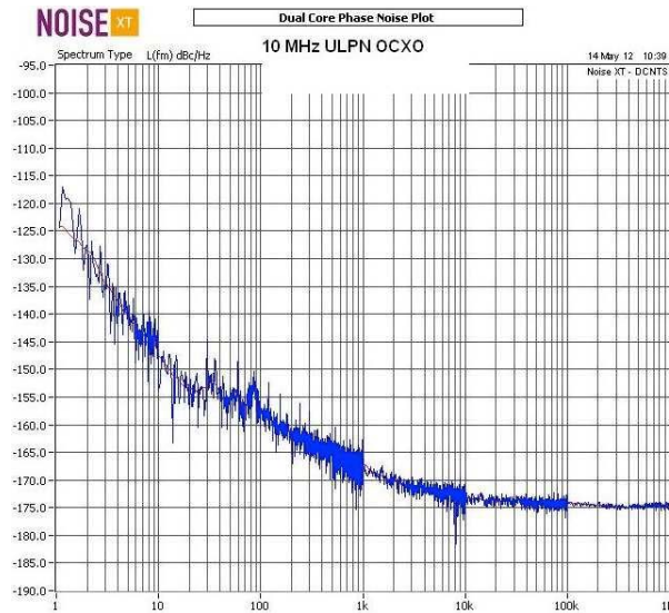
Fig.2. 10.000 MHz ULPN OCXO on DCNTS
