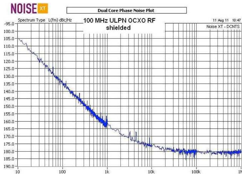
Fig. 5. 100.000 MHz ULPN OCXO phase noise tested with RF-shielded setup.
