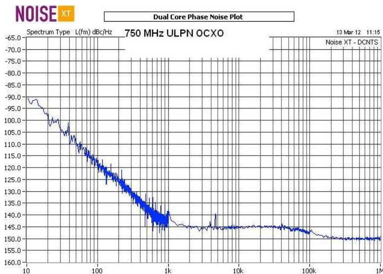
Fig. 10. 750 MHz ULPN OCXO, multiplied from 50 MHz
