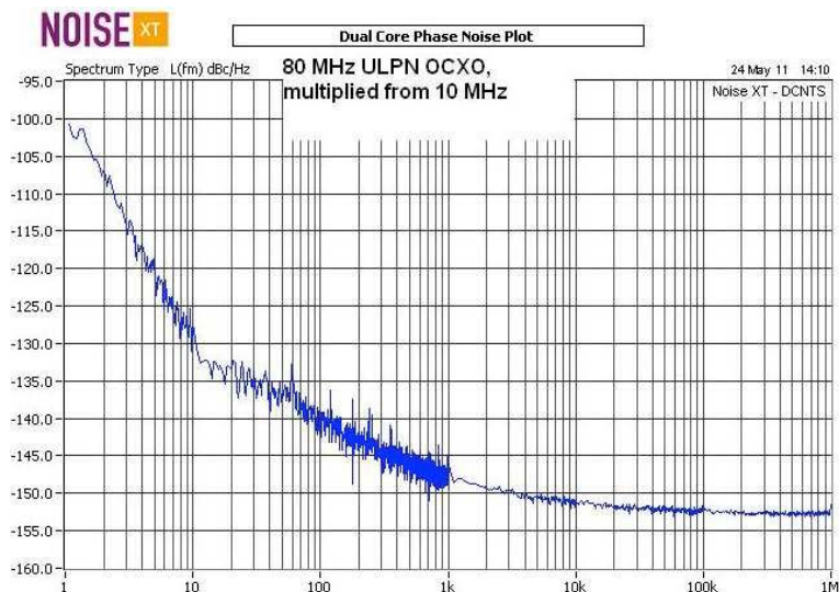
Fig. 9. 80 MHz ULPN OCXO, multiplied from 10 MHz
