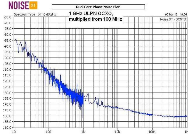
Fig. 11. 1 GHz ULPN OCXO, multiplied from 100 MHz
