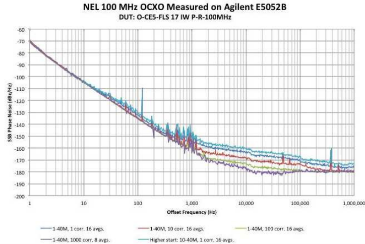
Fig. 7. 100 MHz ULPN OCXO tested on Agilent E5052B with different number of cross-correlations and averages.
