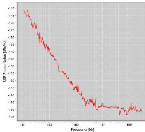
Fig. 8. 100 MHz ULPN OCXO tested on Anapico APPH6000
