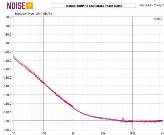
Fig. 6. A batch of 100.000 MHZ ULPN OCXO tests in benign environment. Smooth function is used.
