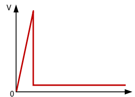
Figure 1.2 I-V Curve of the Switching Overvoltage Protection Component
