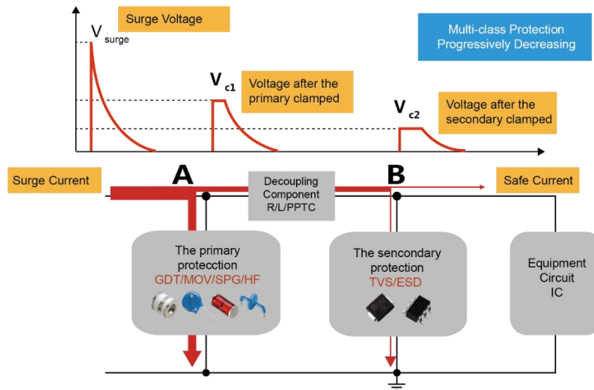
Figure 2.1 Surge protection principle
