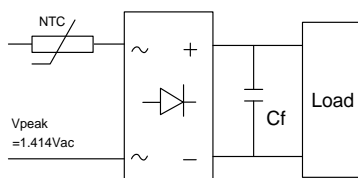
Figure 1.8.4 Full-wave Rectifier
