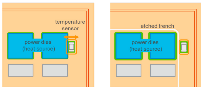
Fig. 3: Substrate geometry and position of the sensor: Distance variations of the sensor (left) and position of the sensor in substrate geometries providing an additional etched trench for insulated sensor positioning (right).
