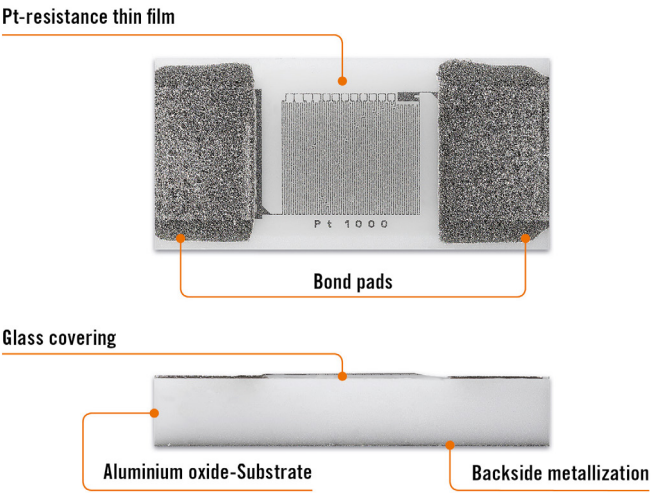
Fig. 1: Components of the sinterable Pt1000 SMD-SC temperature sensor. Bond pads (AgPt) for thin and thick wire bonding and backside metallization (AgPd) optimized for silver sinter processing.
