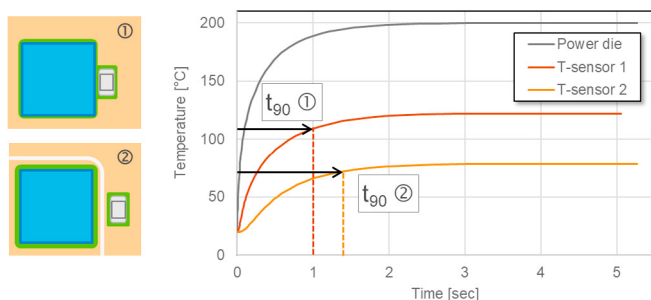
Fig. 6: Dynamics of temperature sensing: temperature response on switch-on process of power dies. Temperature sensor ① is located in proximity to power die, temperature sensor ② is separated from power die by etched trench.
