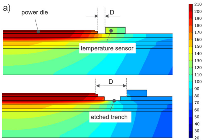
Fig. 5a: Temperature distribution in power modules operated at 200 °C junction temperature. The chosen parameters resemble a SiC-based configuration. Top: substrate geometry without etched trench; Bottom: Additional etched trench for electrically insulated position of the temperature sensor.
