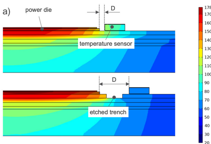
Fig. 4a: Temperature distribution in power modules operated at 150 °C junction temperature. Top: Substrate geometry without etched trench; Bottom: Additional etched trench for electrically insulated position of the temperature sensor.
