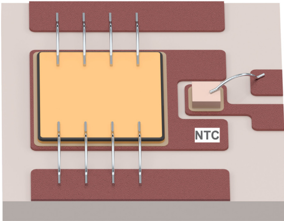
Module setup with NTC Sensor
