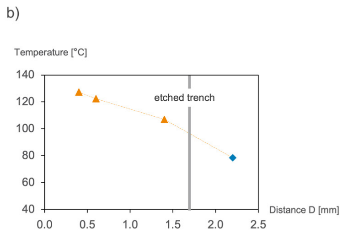
Fig. 5b: Measured temperature as function of the distance between power die and temperature sensor; the position of the additional etched trench is marked as grey double line.
