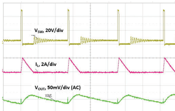
Fig. 33 - Output Ripple 300 mA, Time = 5 \mu\text{s} /div
