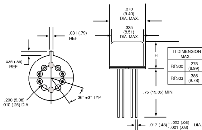
EXTERNAL DIMENSIONS
