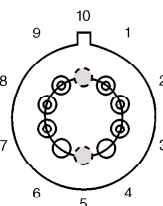
TERMINAL NUMBERING
