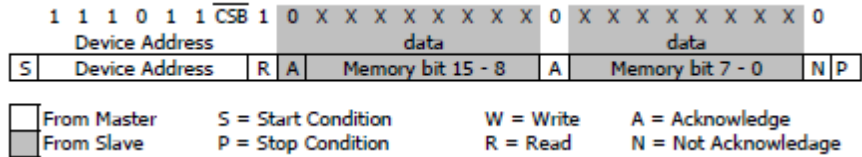
Figure 8: I 2 C answer from MS5803-30BA
