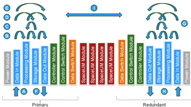
[Figure 1 | The goal of SpaceVPX is to achieve an acceptable level of fault tolerance by way of redundancy and switching. Illustration: VITA.]
