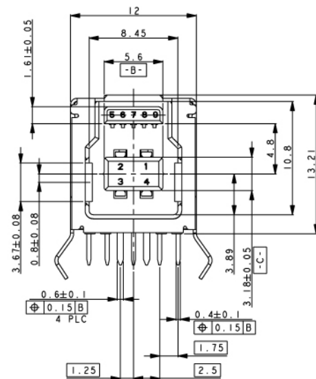
USB 3.0 TYPE RECEPTACLE CONNECTOR
