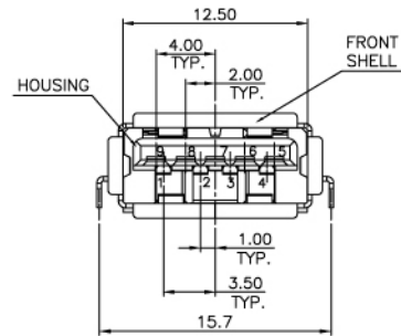
USB 3.0 CONNECTOR STANDARD TYPE A RCPT
