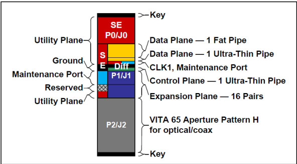
Figure 14.6.11-1 SLT3-PAY-1F1U1S1S1U1U2F1H-14.6.11-n
