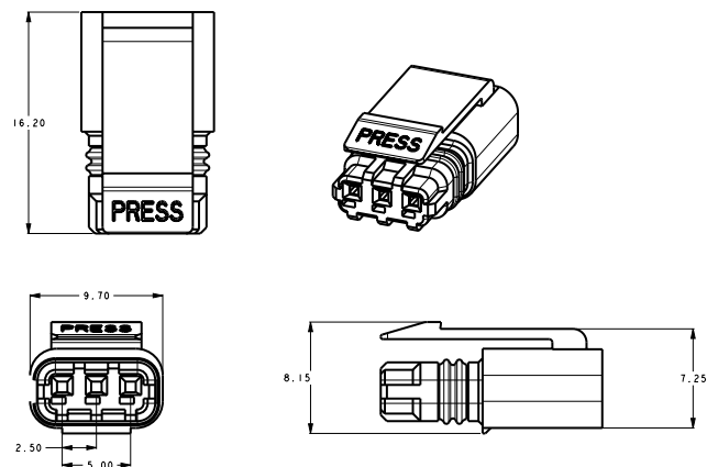
Plug
