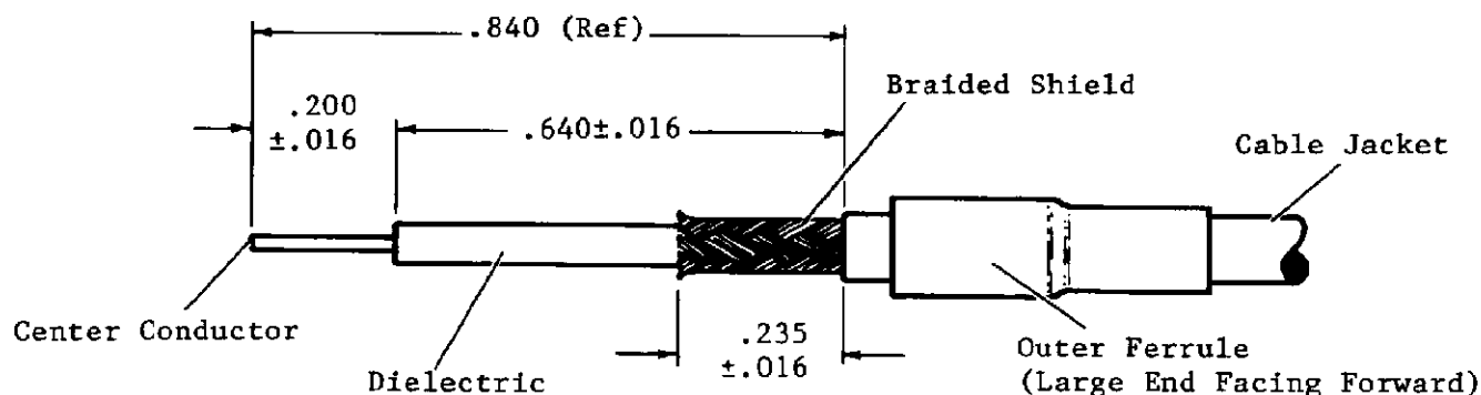
Fig. 4. Cable Strip Lengths
