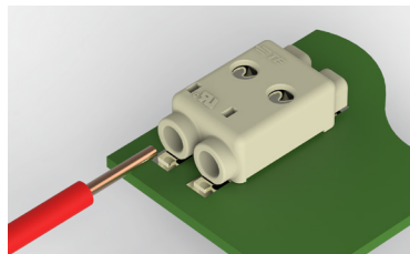
Insert solid conductors horizontal to printed circuit boards to complete termination
