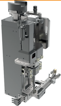
Conversion Kit Mechanical Feed
