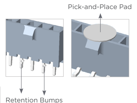
Retention Bumps
