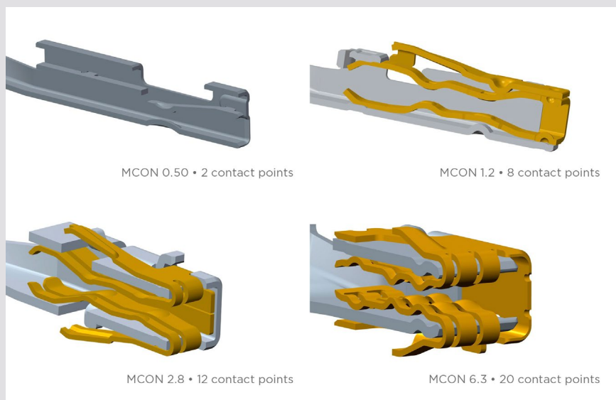
Fig. 2 Two-part design of the MCON receptacle contacts
