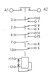
Circuit Configuration 7
