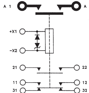
Circuit Configuration 7
