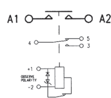
Circuit Configuration 3
