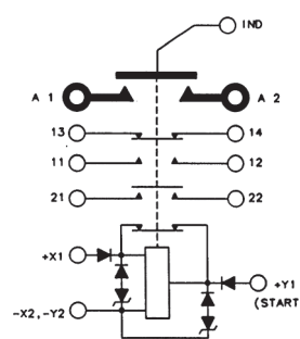
Circuit Configuration 10
