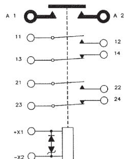
Circuit Configuration 9
