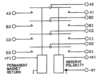
Circuit Configuration 3
