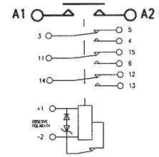
Circuit Configuration 3
