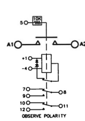
Circuit Configuration 6
