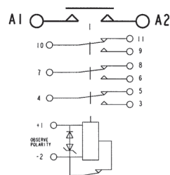
Circuit Configuration 5
