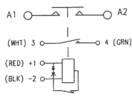
Circuit Configuration 2
