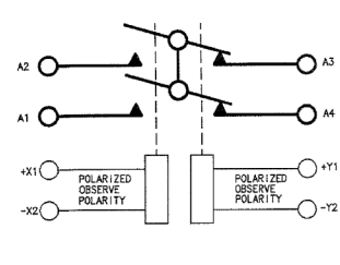
Circuit Configuration 4
