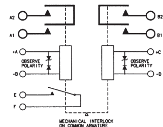
Circuit Configuration 1
