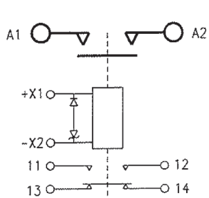
Circuit Configuration 5
