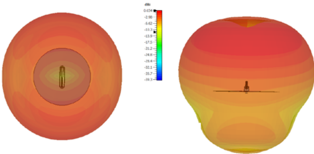
Radiation Patterns at 850 MHz
