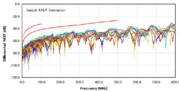
Figure 4. Differential NEXT for CeeLok FAS-T Connector: Single-Connector Link (Source: TE Connectivity)
