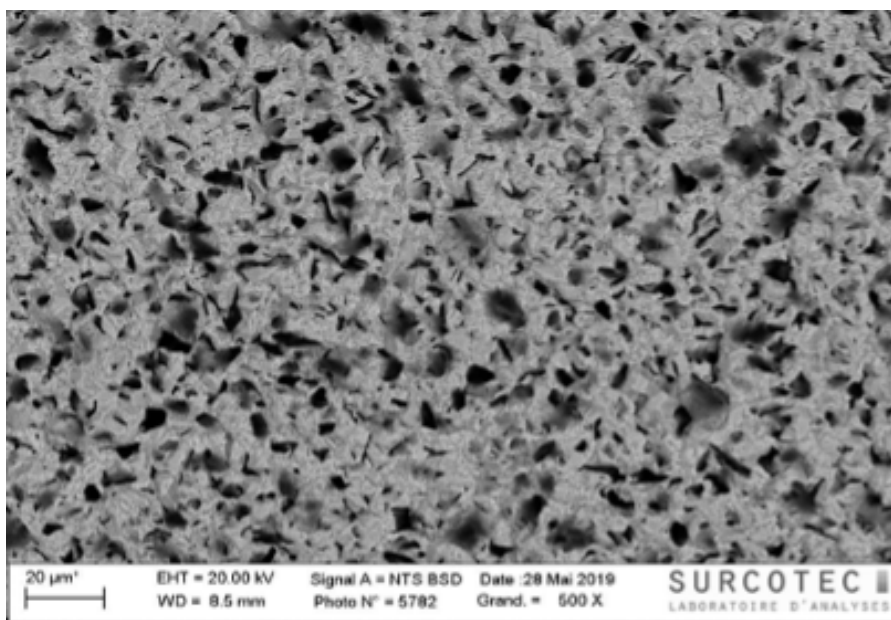
TENDUR ultra abrasion resistant HV contact plating
