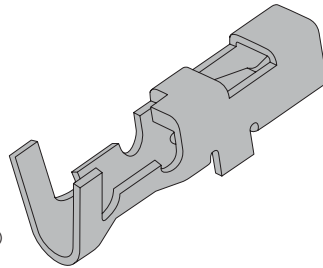
Receptacle Contact (Used on Receptacle Housing)
