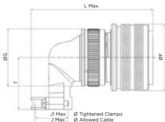
DBAS 976 With Elbowed Cable Clamp
