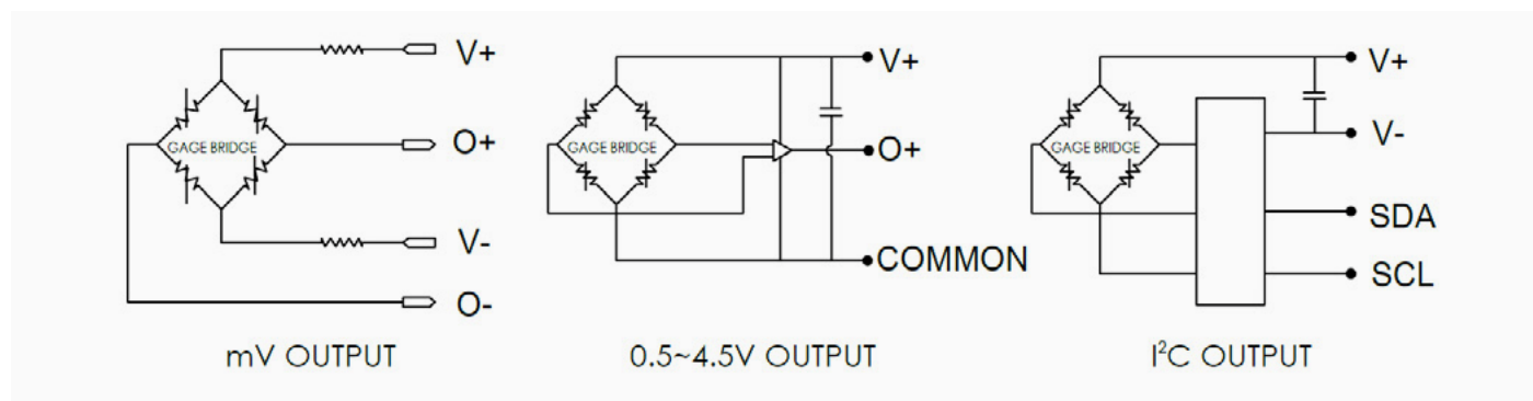
FIGURE 5. OUTPUT SCHEMATICS
