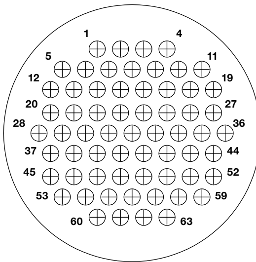
Arrangement 23-63 Max. Wire Ins. Dia. = .068 [1.73]
