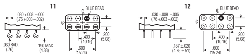
Terminals
