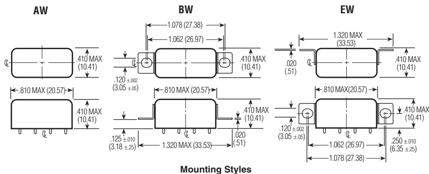
Mounting Styles
