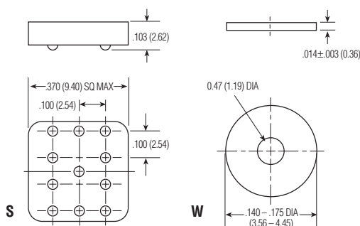
Spreader &amp; Mounting Pads
