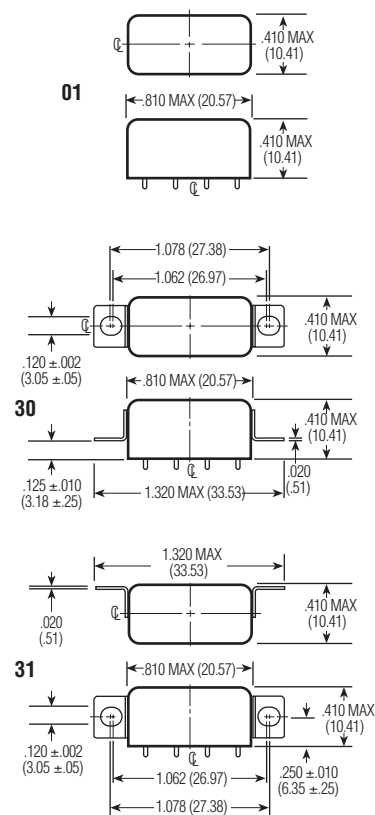
Mounting Styles
