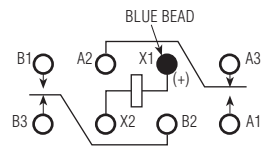
Terminal View
