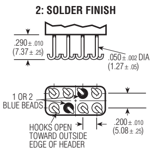
Terminals
