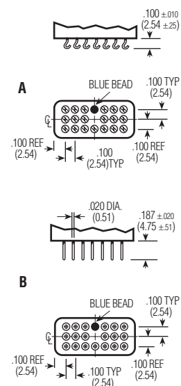
SS Terminals
