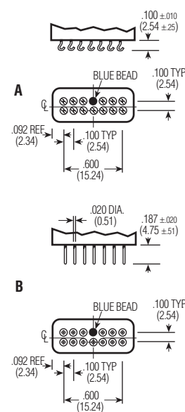
SR Terminals
