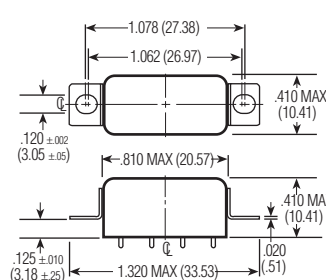
Mounting Styles
