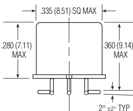
SHC/SHCD Enclosure
