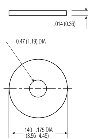
Mounting Pad
