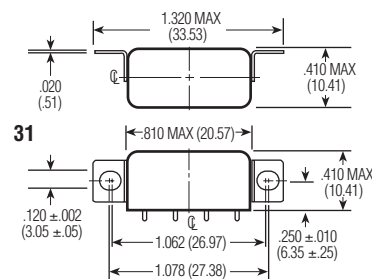
Mounting Styles
