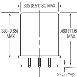
SHCS/SHCSD Enclosure
