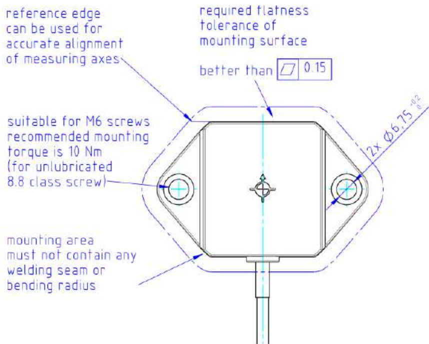
Figure 7. Mounting Detail
