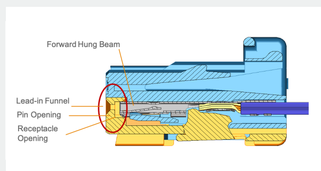
Figure 12: Generation 50 housing
