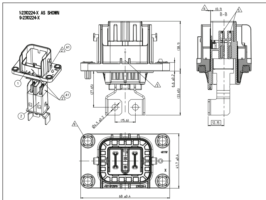
Drawing 2310224
