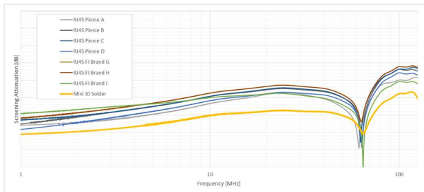
Fig. 6. EMI results
