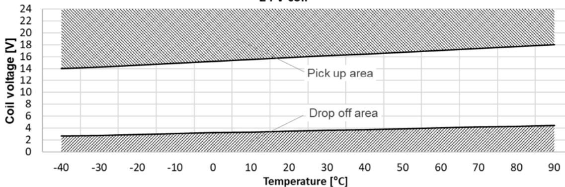
Typical operating voltage characteristics 24 V coil
