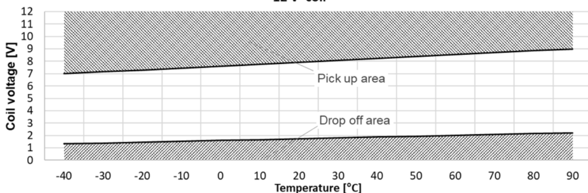
Typical operating voltage characteristics 12 V coil
