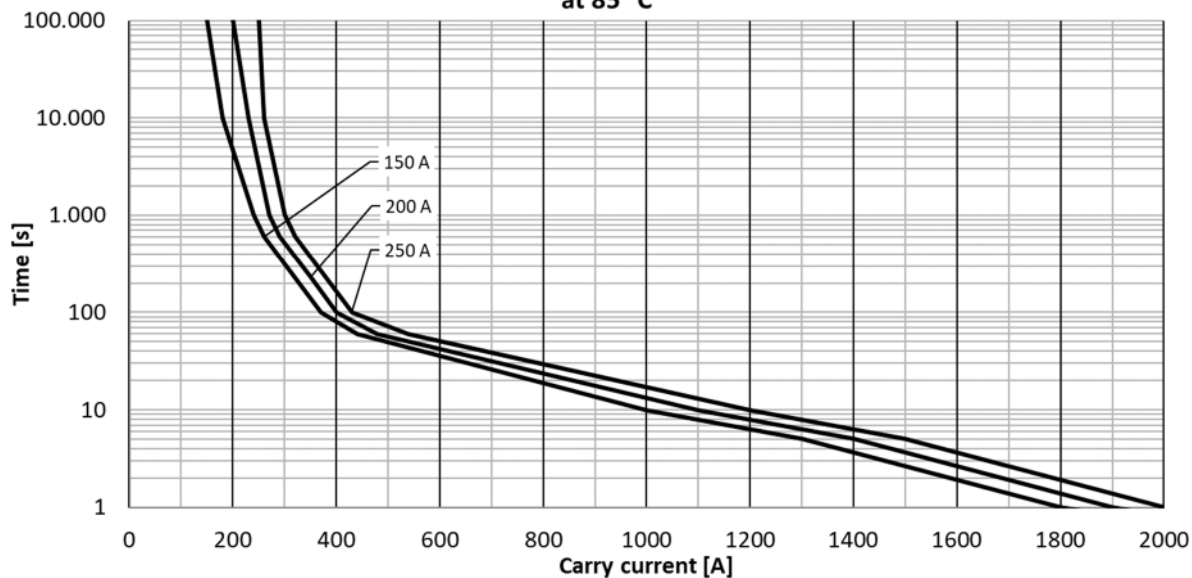
Current handling capability at 85 °C
