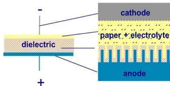
Figure 1: Construction of an aluminum electrolytic capacitor (Source: TDK)
