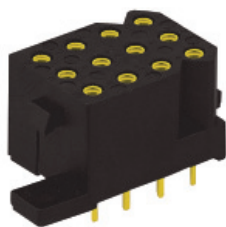
Straight boardmount receptacle delivered with female PCB contacts (SMS GE33)
