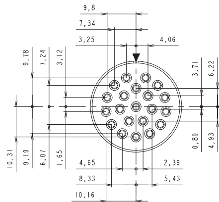
22-21 21 contacts 21 x Ø1.6 (#16)
