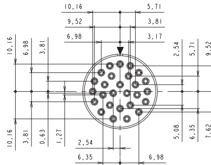
20-27 27 contacts 27 x Ø1.0 (#20)
