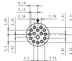
14-15 15 contacts 14 x Ø1.0 (#20) + 1 x Ø1.6 (#16)
