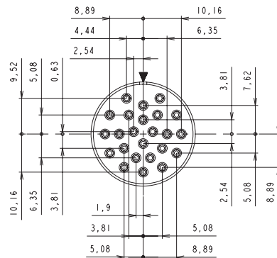
20-24 24 contacts 24xØ1.0 (#20)
