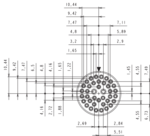
20-39 39 contacts 37 x Ø1.0 (#20) + 2 x Ø1.6 (#16)
