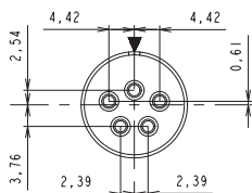
14-5 5 contacts 5 x Ø1.6 (#16)
