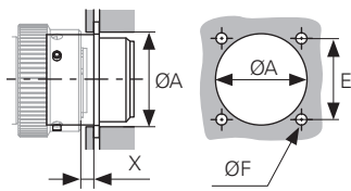
Square flange receptacle
