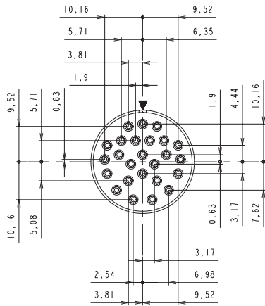
20-25 25 contacts 25 x Ø1.0 (#20)
