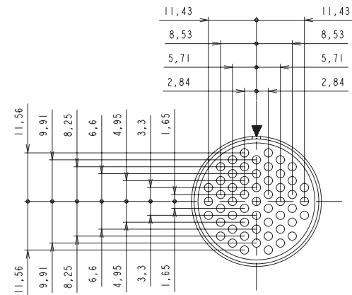
22-55 55 contacts 55 x Ø1.0 (#20)
