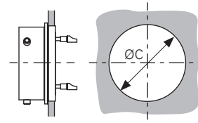
Solder fixing receptacle
