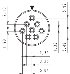
16-8 8 contacts 8 x Ø1.6 (#16)
