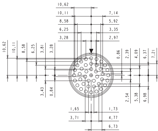
20-41 41 contacts 41 x Ø1.0 (#20)
