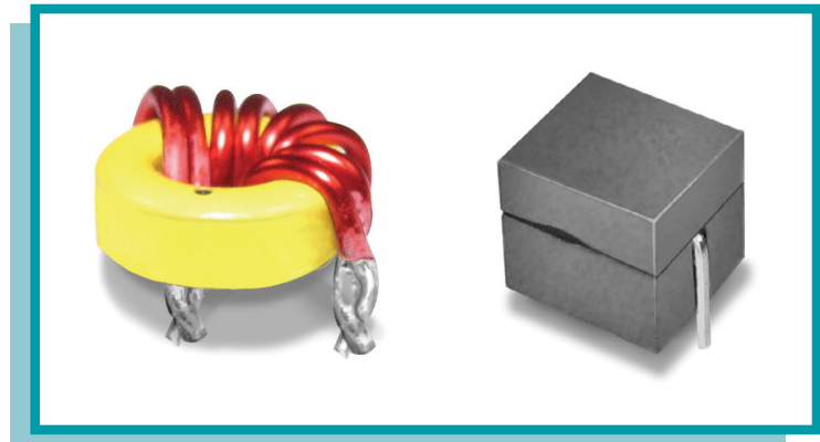
Fig. 1. Historically, wound-toroid inductors used in microprocessor core voltage regulators employed low-cost, high-permeability powdered-iron cores.
