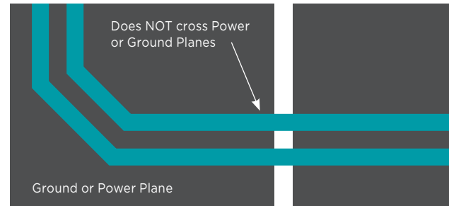
Figure 4. Differential Signal Pair-Plane Crossing
