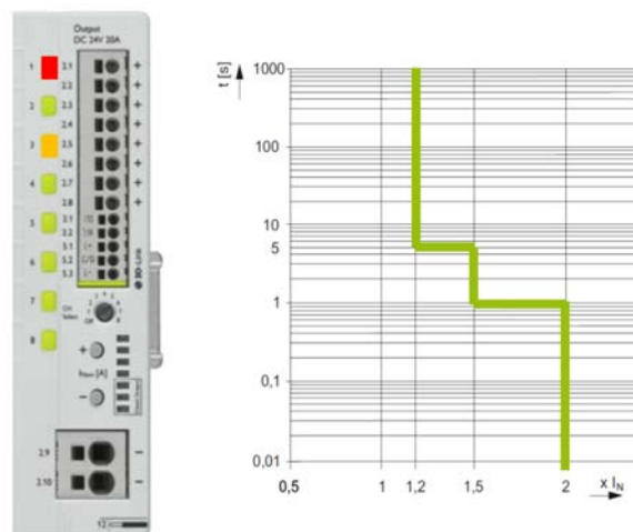
Figure 3: Multicolor LED (left) and tripping characteristics (right) of the TRIO3 with integrated circuit breakers.
