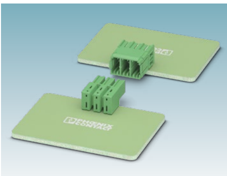
PC 5 PCB connectors with 7.62 mm pitch for currents up to 41 A per contact for wave soldering.
