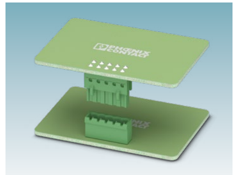
MSTB 2,5 PCB connectors with 5.08 and 7.62 mm pitch for currents up to 16 A per contact for wave soldering.
