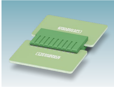
ZEC 1,0 / 1,5 PCB connectors for direct plug-in with 3.5, 5.0, and 7.5 mm pitch for currents up to 10 A per contact.
