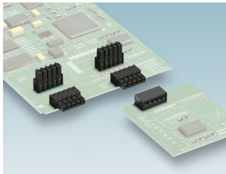
MC 1,5 PCB connectors with 3.5 and 3.81 mm pitch for currents up to 8 A per contact for THR and wave soldering.
