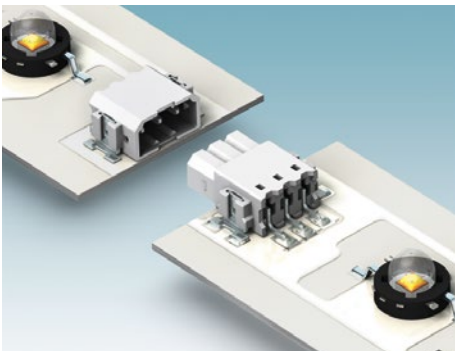
PTSM 0,5 THR and SMD PCB connectors with 2.5 mm pitch for currents up to 6 A per contact.
