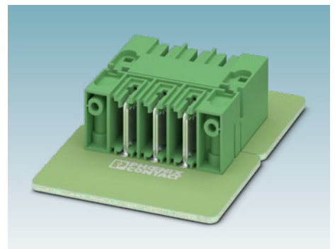
PC 35 PCB connectors with 15 mm pitch for currents up to 125 A per contact for wave soldering.
