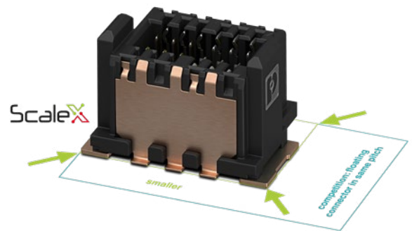
Space requirement compared that of a common floating connector
