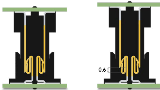
Minimum and maximum PCB clearance with wiper length
