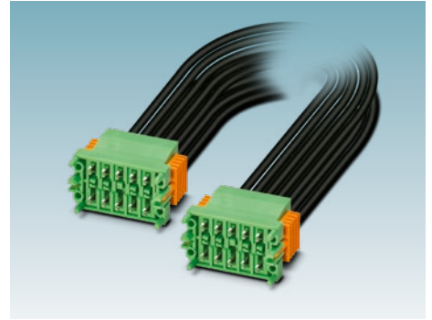
CDDC 1,5 / 2,5 Pre-assembled PCB connectors for direct plug-in with pitches of 3.5 mm and 5.0 mm currents of up to 12 A per contact.
