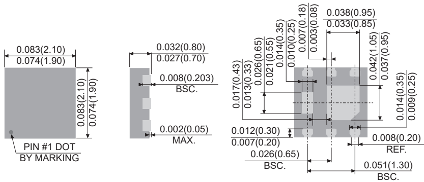
DFN2020-8L
