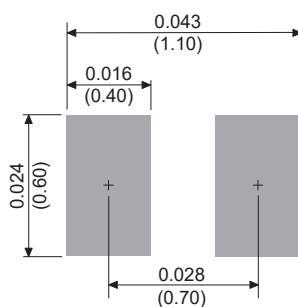
DFN1006-2L
