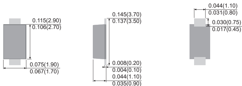
SOD-123FL
