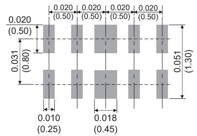
DFN2510A-10L
