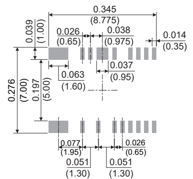
TSSOP-18
