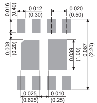
DFN2020-8L
