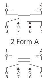
Schematic ( BOTTOM VIEW ) ( De-energize ) 1 Form A 1 Form B
