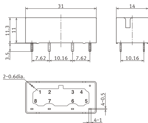
External dimensions
