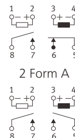
Schematic ( BOTTOM VIEW ) ( Reset ) 1 Form A 1 Form B
