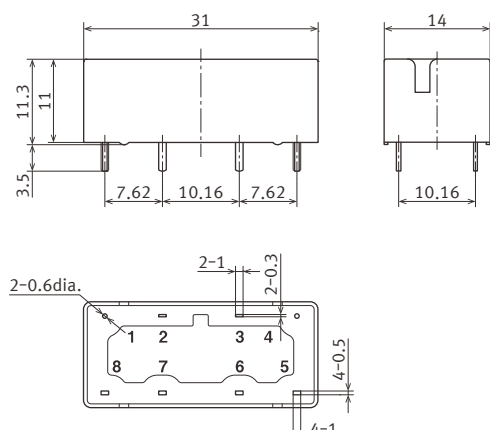
External dimensions
