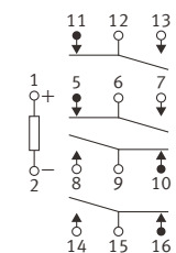
2 coil latching ( Reset )
