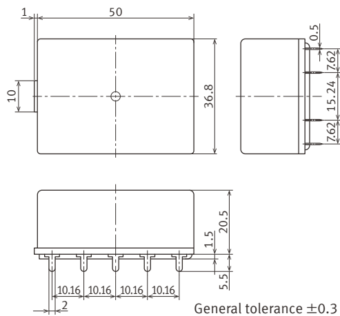
External dimensions
