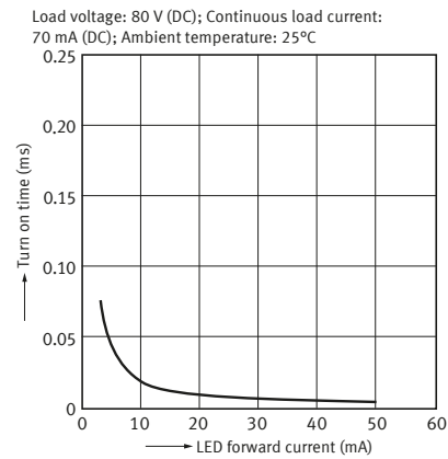
10. Turn on time vs. LED forward current characteristics
