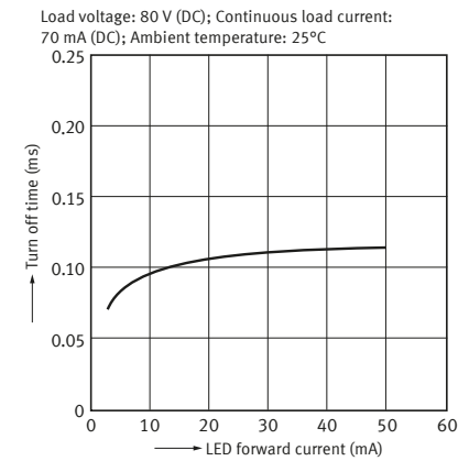
11. Turn off time vs. LED forward current characteristics
