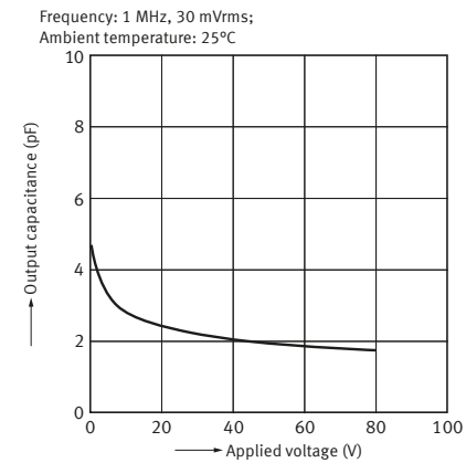
12. Output capacitance vs. applied voltage characteristics
