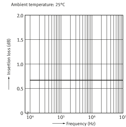
14. Insertion loss vs. frequency characteristics ( 50 Ω impedance )
