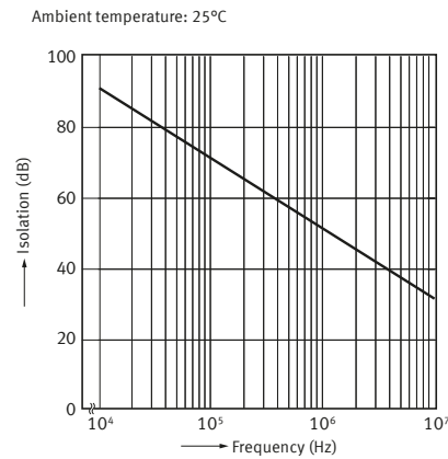
13. Isolation vs. frequency characteristics ( 50 Ω impedance )
