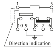
1 coil latching ( Reset )
