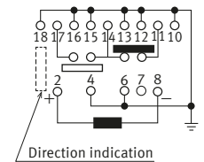
2 coil latching ( Reset )
