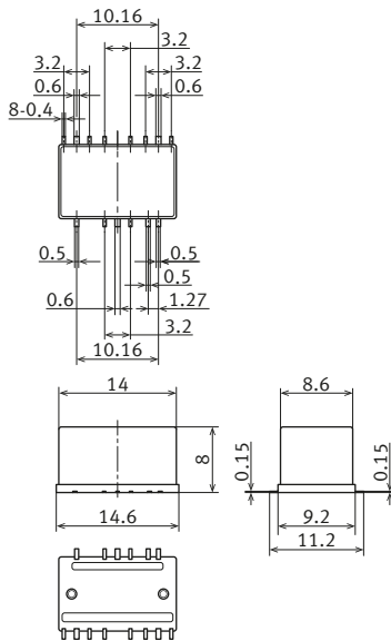
External dimensions
