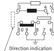
2 coil latching ( Reset )
