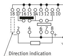
1 coil latching ( Reset )
