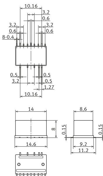
External dimensions
