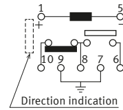
2 coil latching ( Reset )
