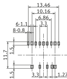
Recommended PC board pattern ( TOP VIEW ) 50 Ω
