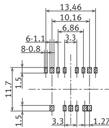
Recommended PC board pattern ( TOP VIEW ) 50 \Omega
