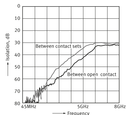
Isolation characteristics
