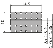
Calibration board
