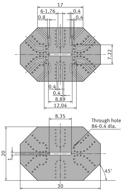
Surface mount terminal
