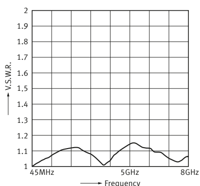
V.S.W.R. characteristics
