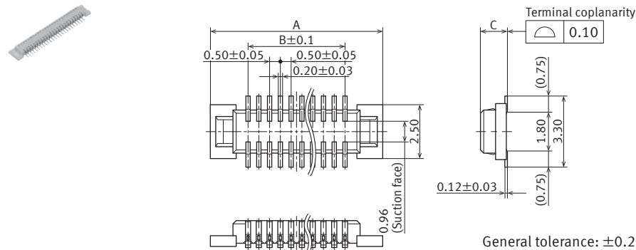
External dimensions
