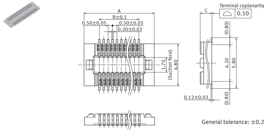
External dimensions
