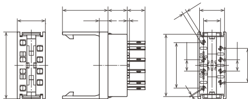
External dimensions
