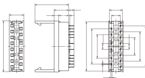
External dimensions
