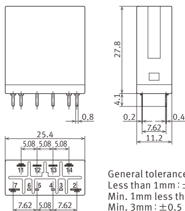
External dimensions
