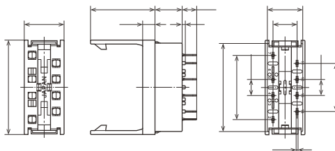
External dimensions
