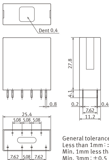
External dimensions
