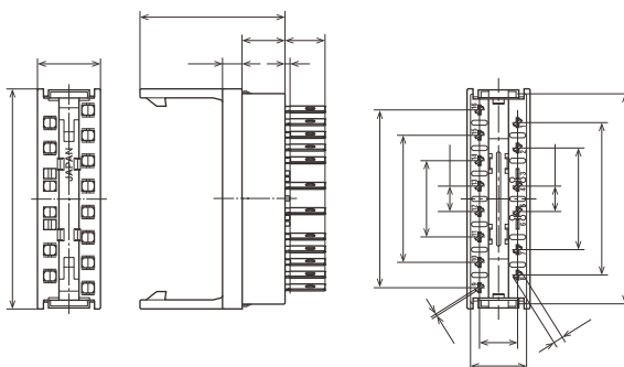
External dimensions
