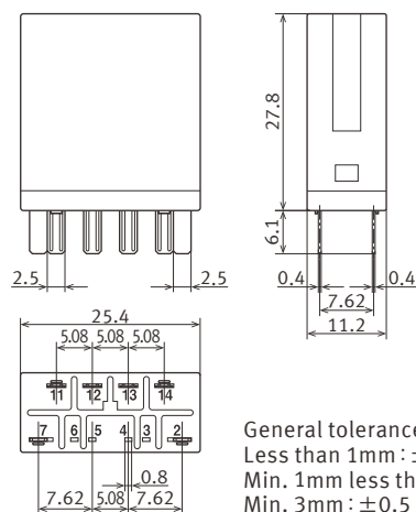
External dimensions
